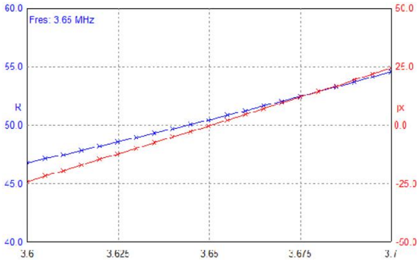
Figure 5 Z of the Inverted L Antenna for 80- meter Band
