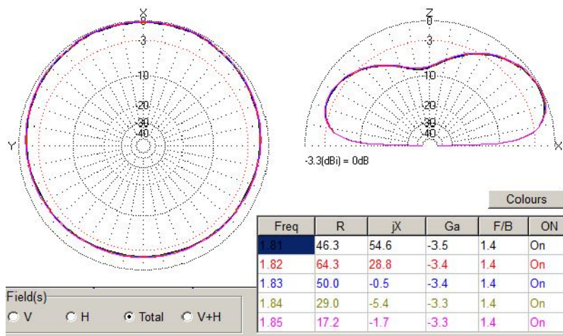
Figure 4 DD of the Inverted L Antenna for 160- meter Band
