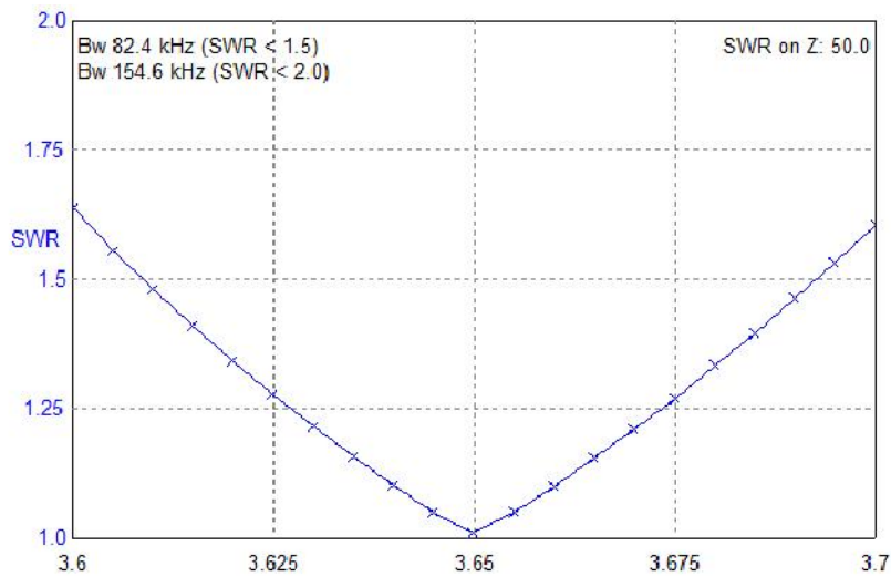
Figure 6 SWR of the Inverted L Antenna for 80- meter Band
