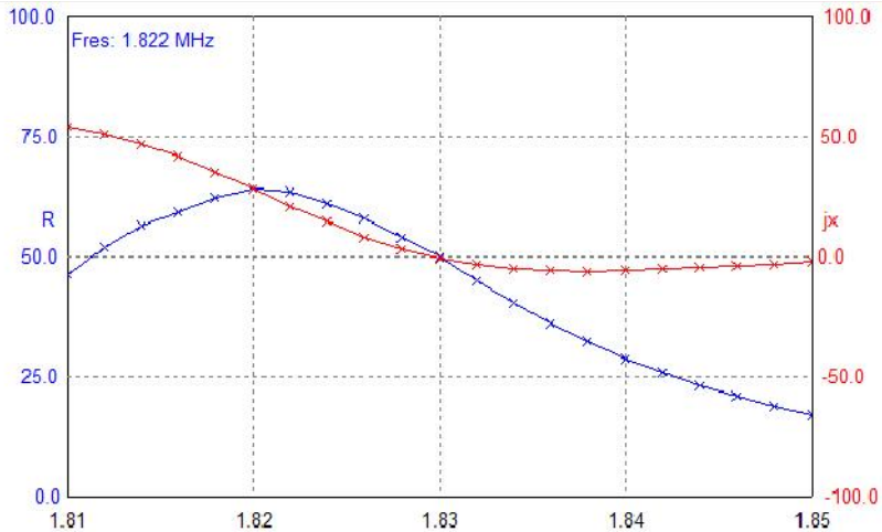
Figure 2 Z of the Inverted L Antenna for 160- meter Band
