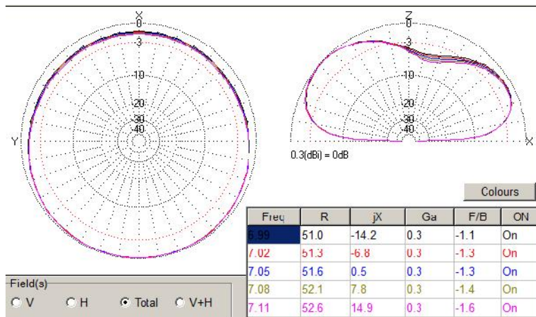
Figure 10 DD of the Inverted L Antenna for 40- meter Band
