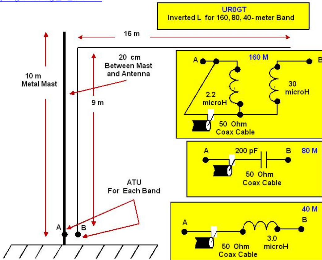
Figure 1 Inverted L Antenna for 160, 80 and 40- meter Band
