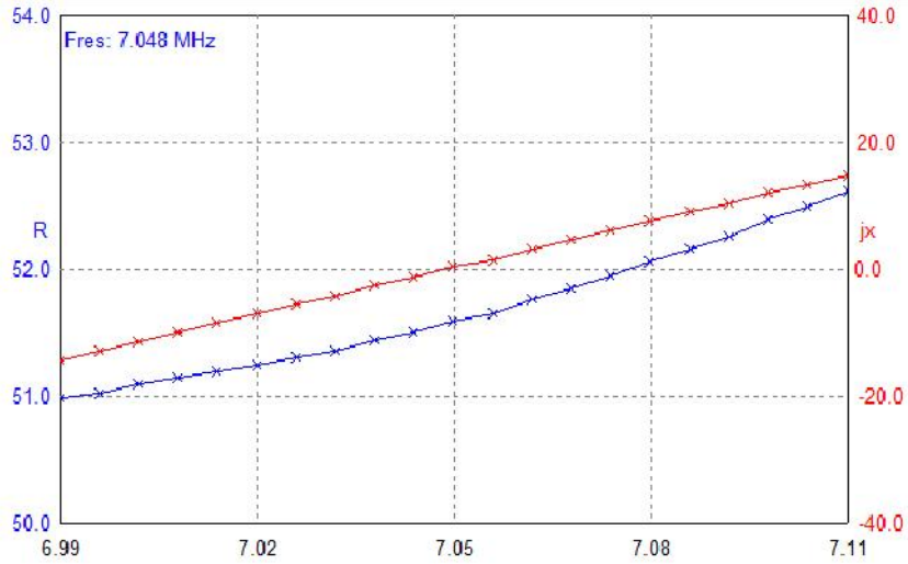
Figure 8 Z of the Inverted L Antenna for 40- meter Band
