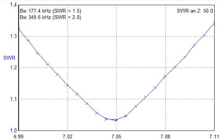
Figure 9 SWR of the Inverted L Antenna for 40- meter Band
