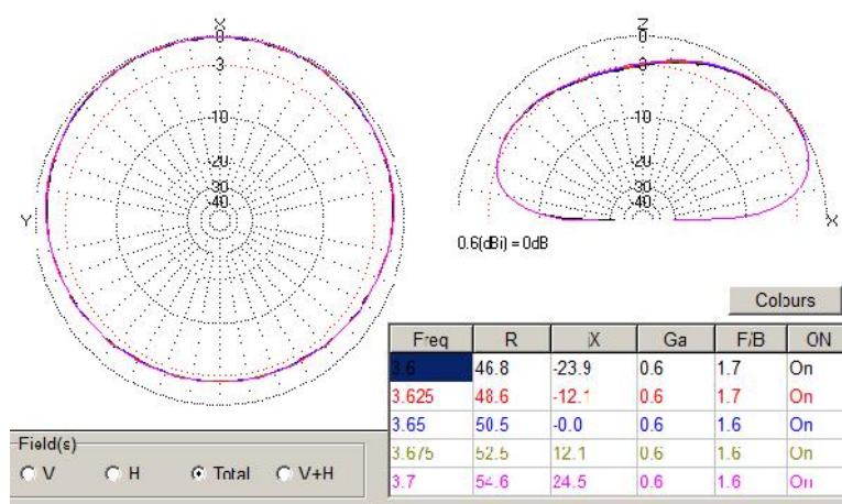
Figure 7 DD of the Inverted L Antenna for 80- meter Band
