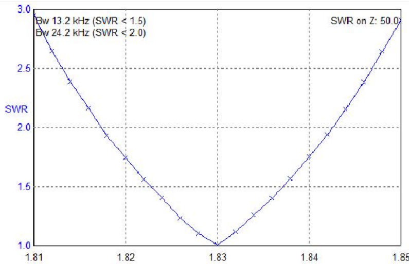
Figure 3 SWR of the Inverted L Antenna for 160- meter Band
