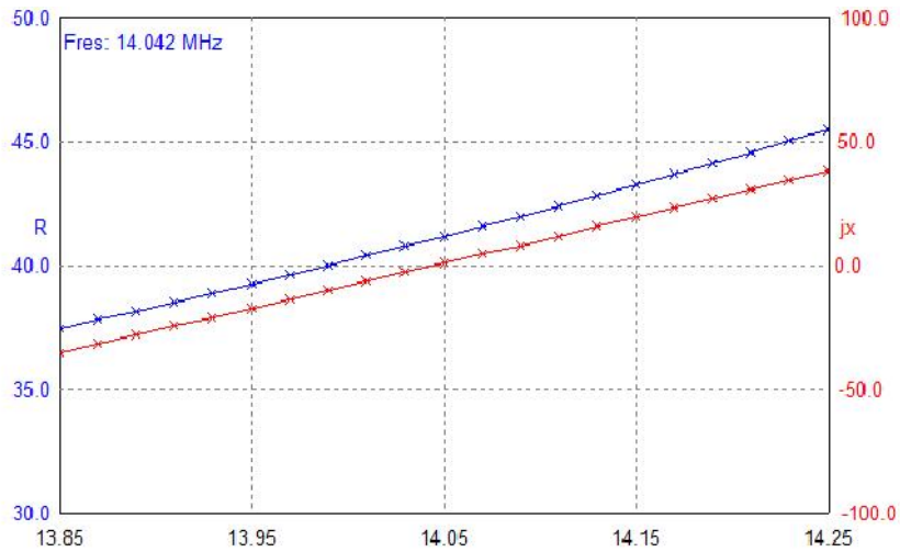
Figure 5 Z of the Compact Dipole Antenna for the 40- and 20- meter Band at 20- meter Band
