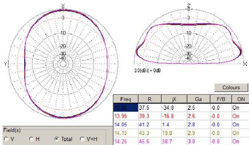
Figure 7 DD of the Compact Dipole Antenna for the 40- and 20- meter Band at 20- meter Band
