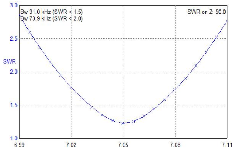
Figure 3 SWR of the Compact Dipole Antenna for the 40- and 20- meter Band at 40- meter Band
