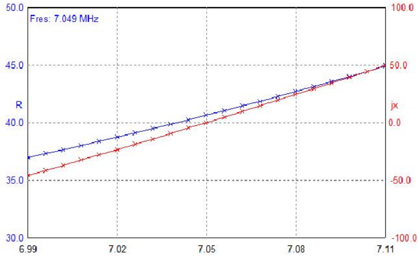
Figure 2 Z of the Compact Dipole Antenna for the 40- and 20- meter Band at 40- meter Band
