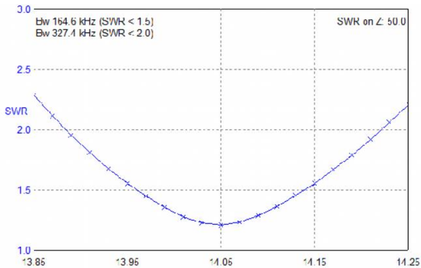
Figure 6 SWR of the Compact Dipole Antenna for the 40- and 20- meter Band at 20- meter Band
