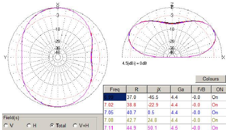
Figure 4 DD of the Compact Dipole Antenna for the 40- and 20- meter Band at 40- meter Band
