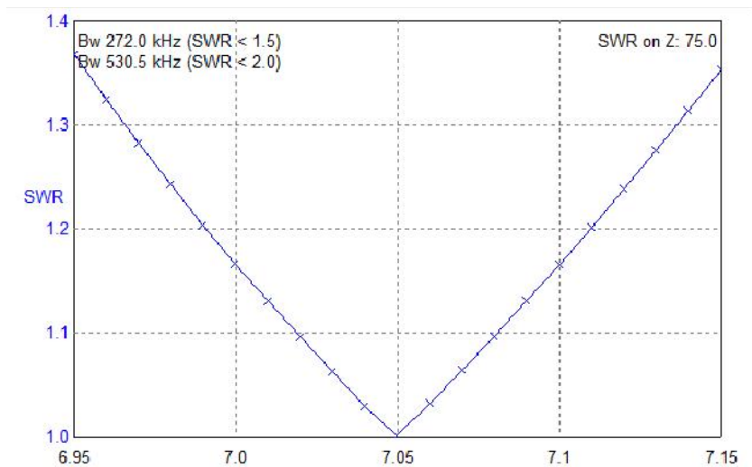
Figure 3 SWR of the Simple Dipole Antenna for 7 and 21- MHz Band at 7-MHz Band
