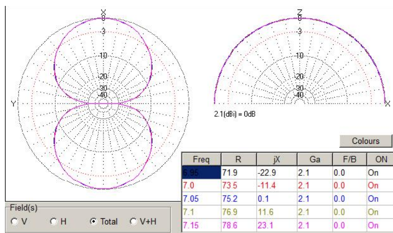
Figure 4 DD of the Simple Dipole Antenna for 7 and 21- MHz Band at 7-MHz Band
