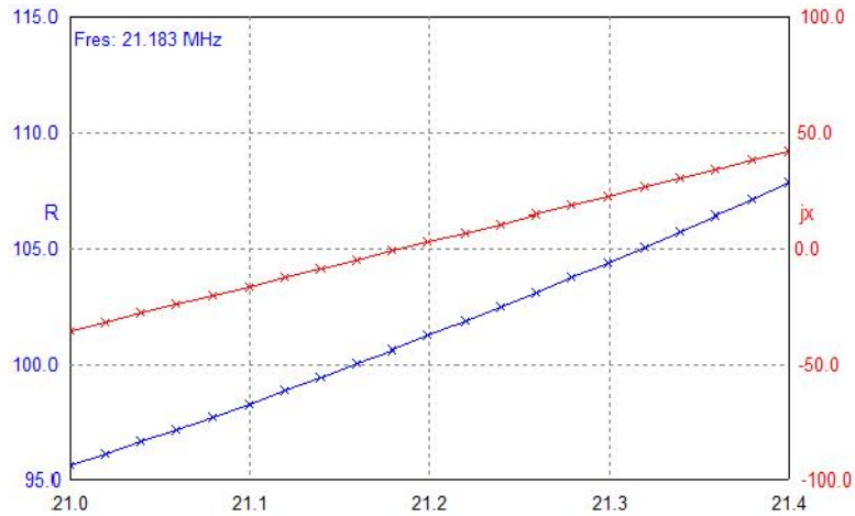
Figure 5 Z of the Simple Dipole Antenna for 7 and 21- MHz Band at 21-MHz Band
