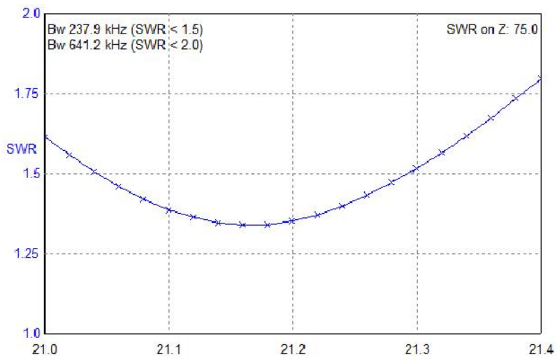
Figure 6 SWR of the Simple Dipole Antenna for 7 and 21- MHz Band at 21-MHz Band
