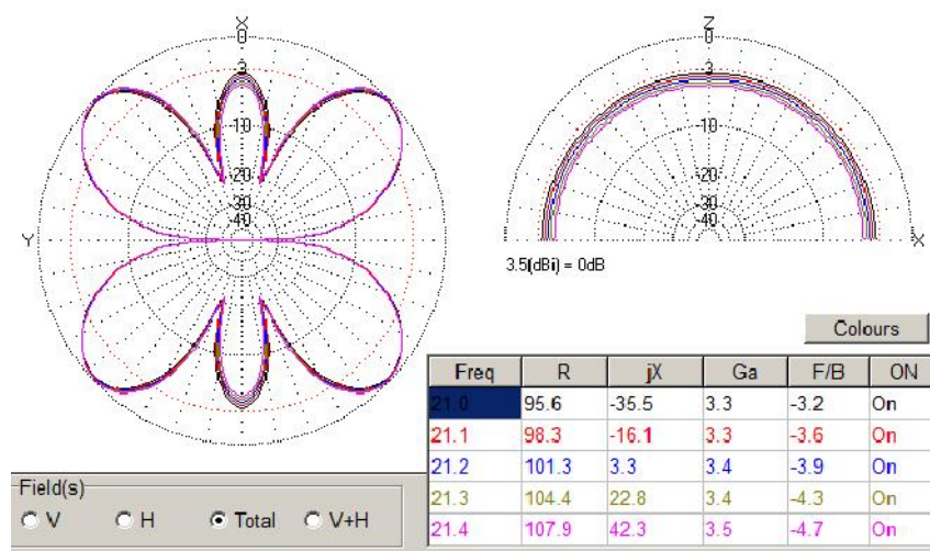
Figure 7 DD of the Simple Dipole Antenna for 7 and 21- MHz Band at 21-MHz Band
