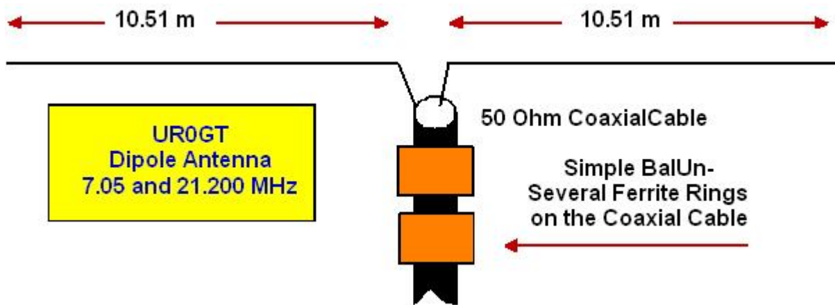
Figure 1 Simple Dipole Antenna for 7 and 21- MHz Band
