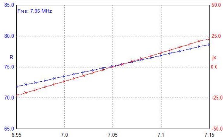
Figure 2 Z of the Simple Dipole Antenna for 7 and 21- MHz Band at 7-MHz Band
