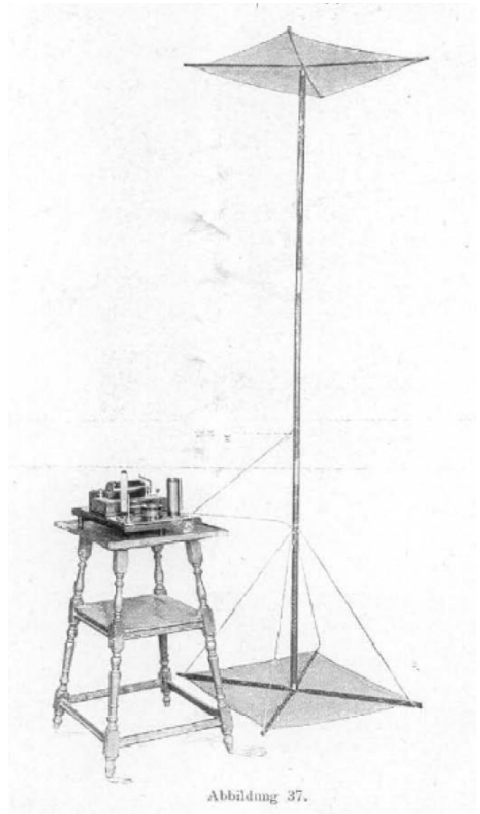
Field Receiver with Field Antenna Telefunken Catalog from 1919
