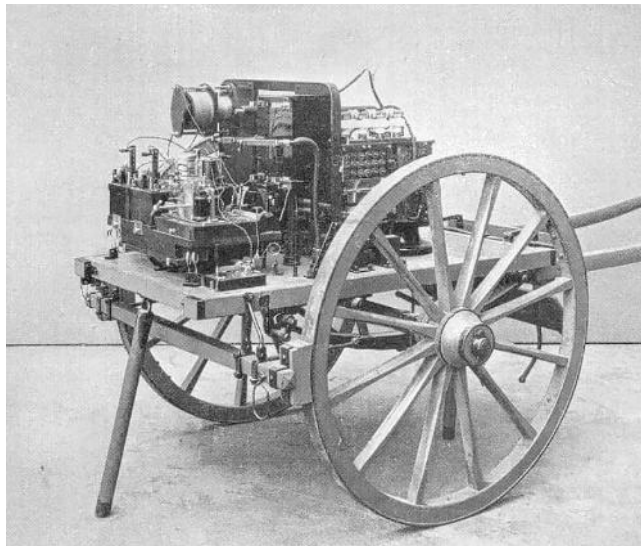
Field Receiver / Transmitter on a Horse Cart Telefunken Catalog from 1919
