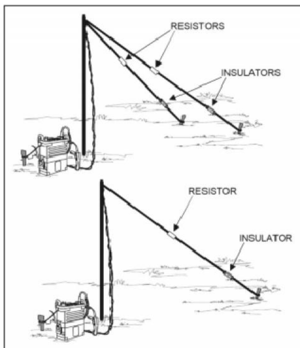
Figure 9-16. Sloping-V antenna
