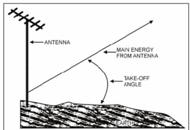
Figure 9-7. Antenna take-off angle
