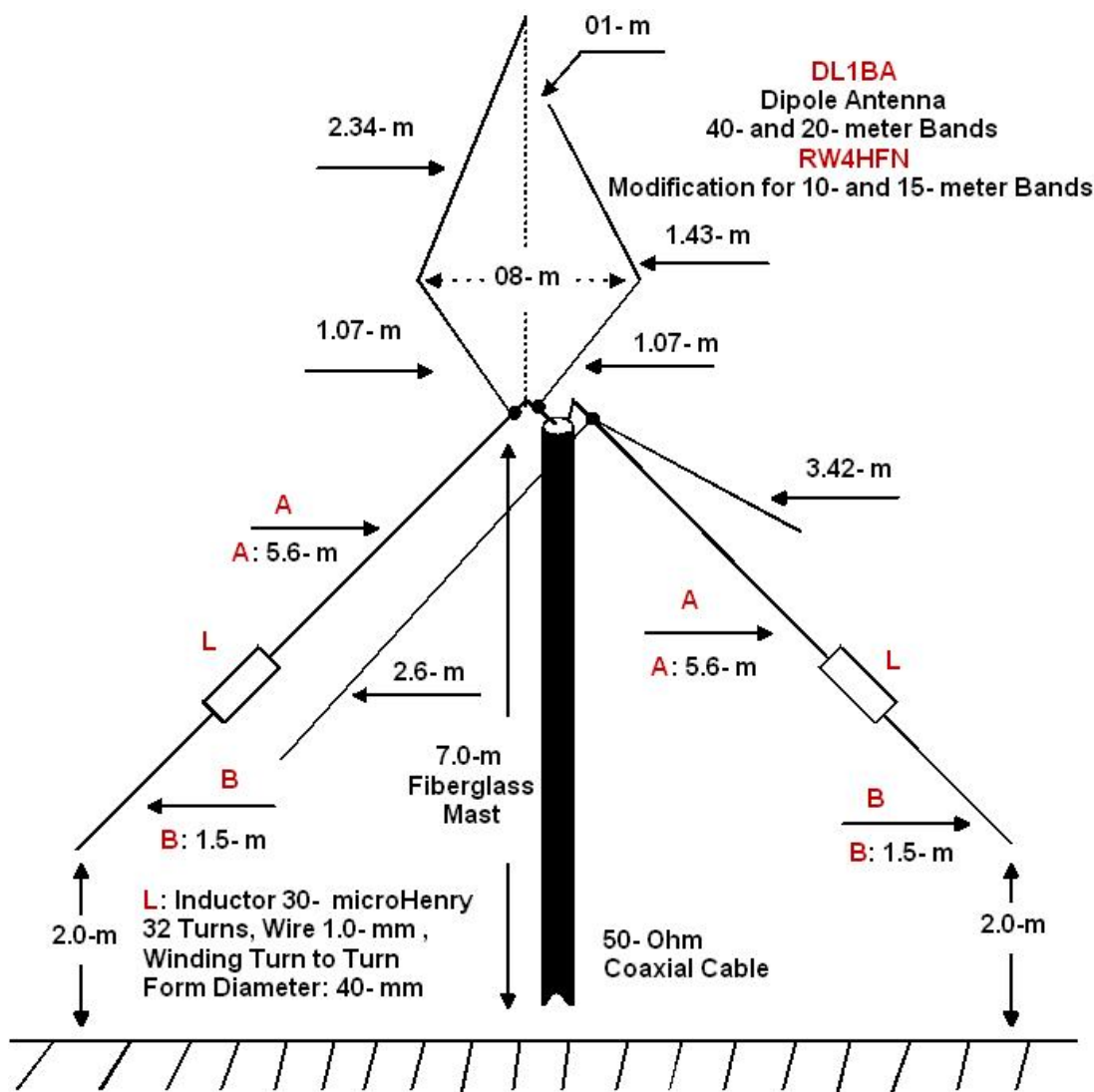
Figure 1 Modified DL1BA Dipole Antenna for 40-, 20-, 15-, and 10- meter Bands
