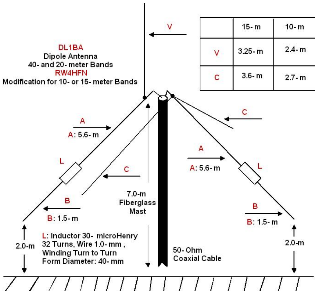
Figure 1 Modified DL1BA Dipole Antenna for 40- and 20- meter Bands with Additional 10- or 15- meter Band
