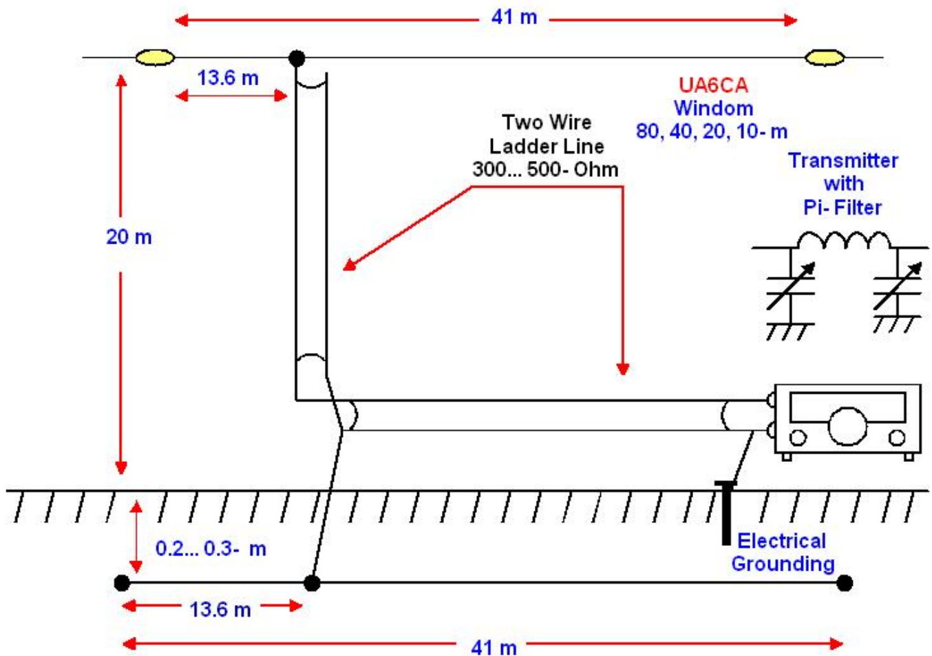
Figure 1 Windom UA6CA for 80-, 40-, 20- and 10- meter Bands
