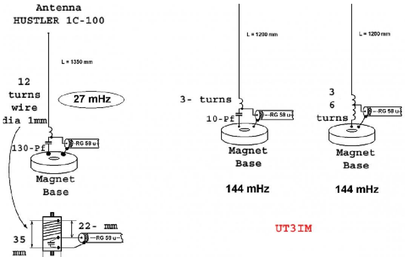
Figure 1 Conversion Auto CB-Antenna HUSTLER-1C-100 to Antenna for the 2- meter Band
