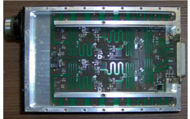
at the front side there was a board with VHF circuit. The resonators made from silvered bronze.
