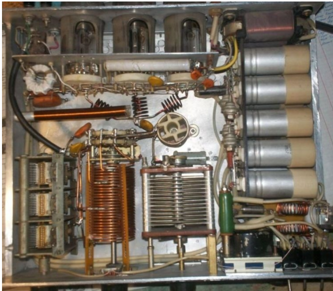
P.A. 3 x GU- 50 Picture by US5ITP
