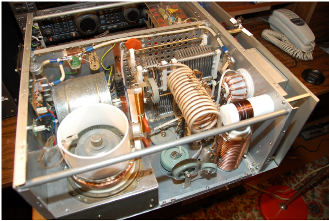
P.A. on GU-84B Picture by RA3DNC
