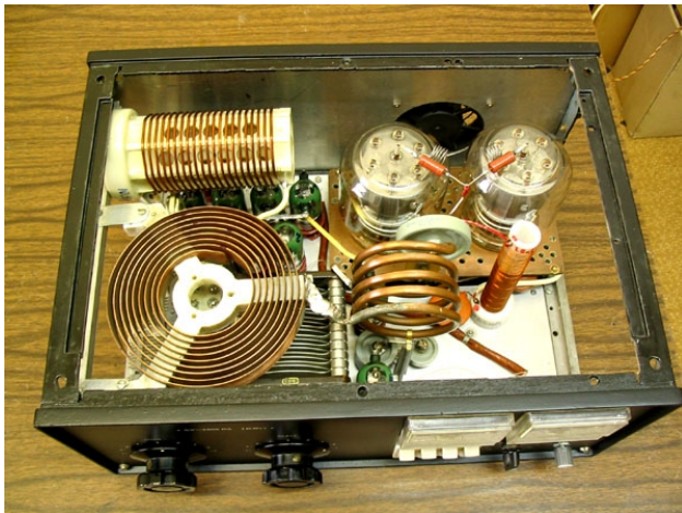
Inductor in one plane Picture by UN7RX
