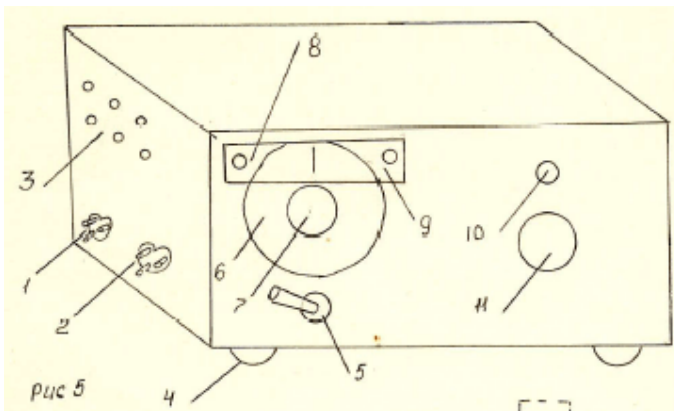
Transceiver TST
